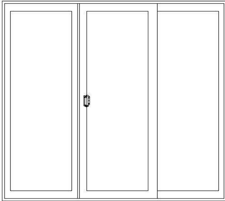
7668 (89-1/2" x 79-1/2") Left or Right (OXO)
