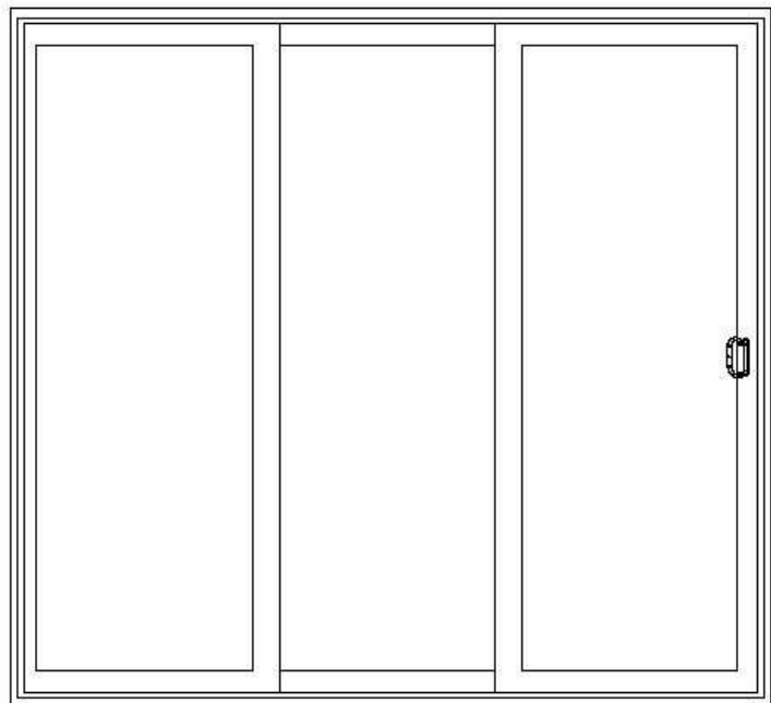
7668 (86-1/2" x 79-1/2") Left or Right (OOX)
