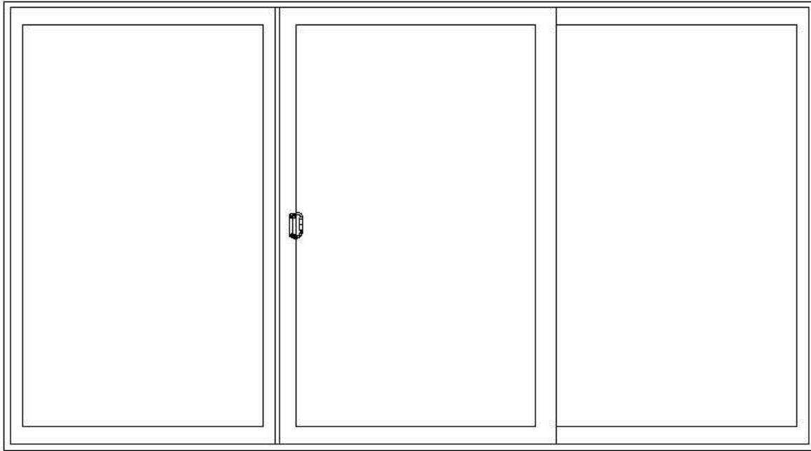
12068 (143-1/2" x 79-1/2") Left or Right (OXO)
