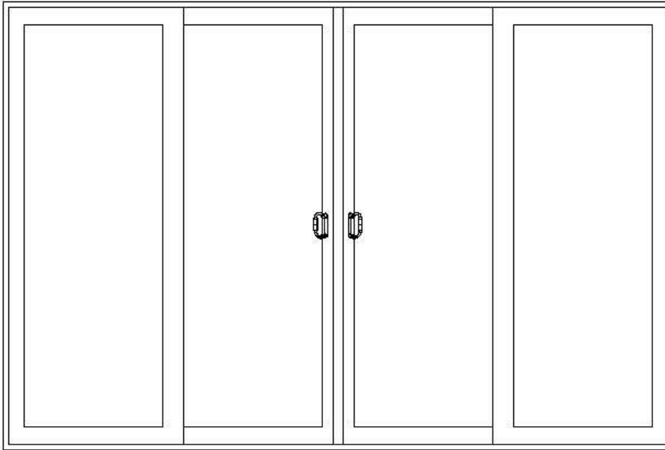
10068 (118-1/4" x 79-1/2") Left or Right Primary (OXXO)
