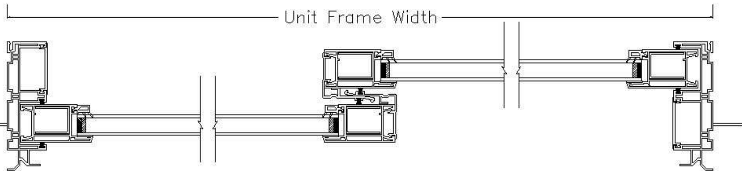
HORIZONTAL SECTION B-B
